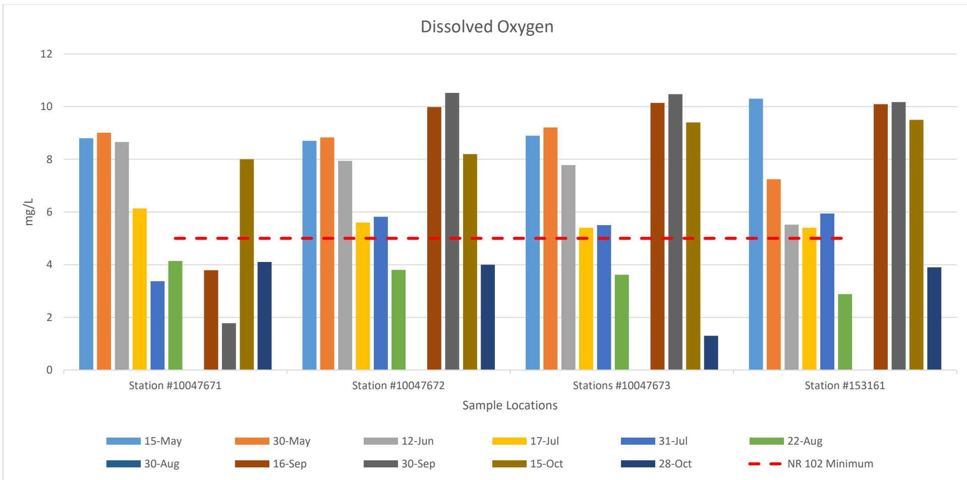
Chart 5-5. Dissolved Oxygen Concentrations in Upstream Samples
