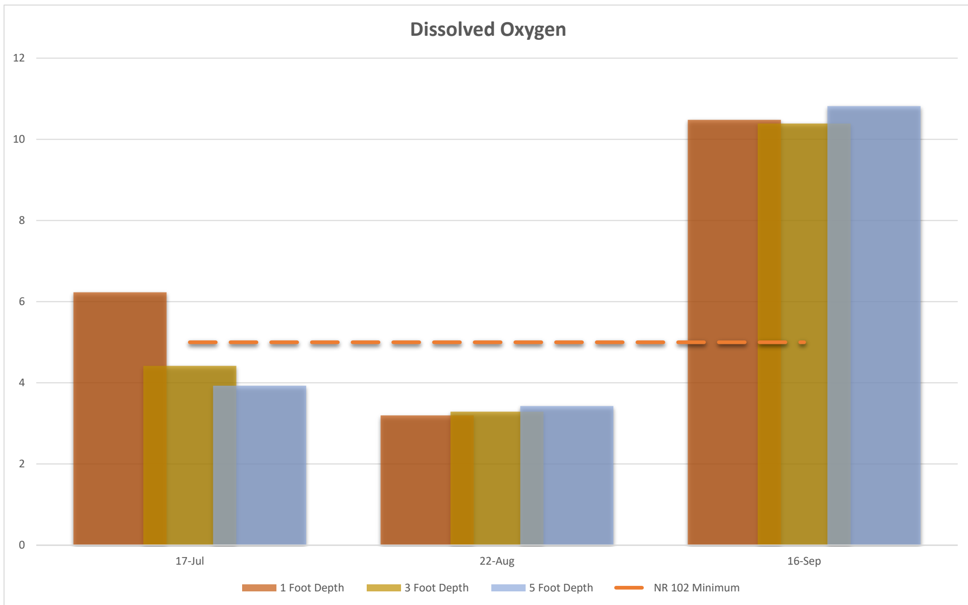
Chart 5-6. Dissolved Oxygen Concentrations in Millpond Samples
